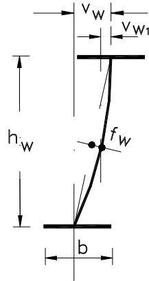
Figure (12.3) Deviations in Welded Girders
