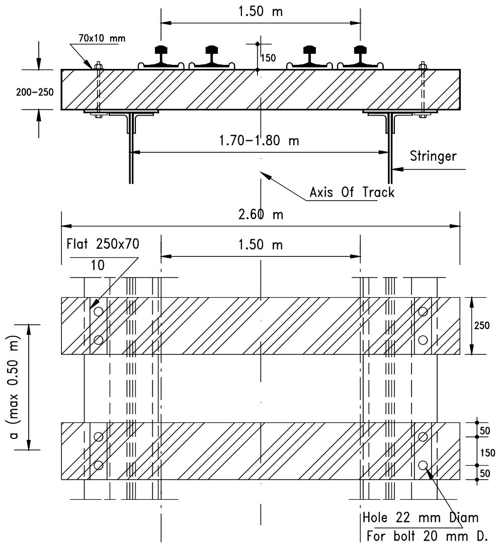
Figure (9.5) Fixation of Sleepers on Steel Bridges
