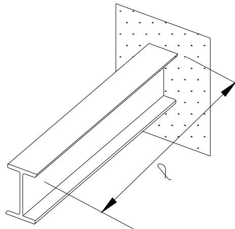
Figure (4.5) Continuous Cantilever with Lateral and Torsional Restraint
