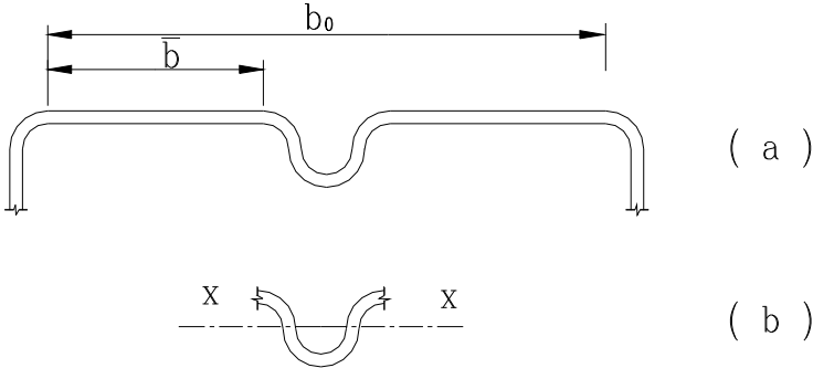
Figure (11.4) Elements with Intermediate Stiffener
