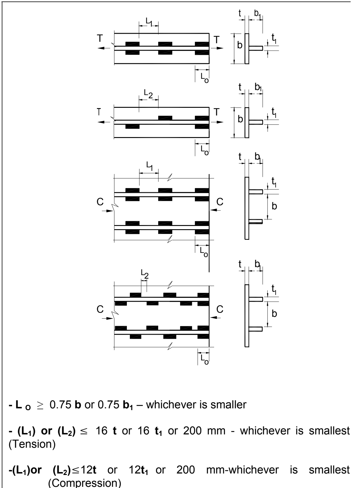
Figure (5.12) Intermittent Fillet Welds
