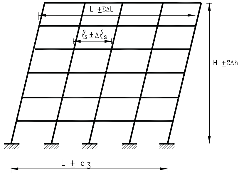
Figure (12.9) Deviation in Length ( Vertical Section )
