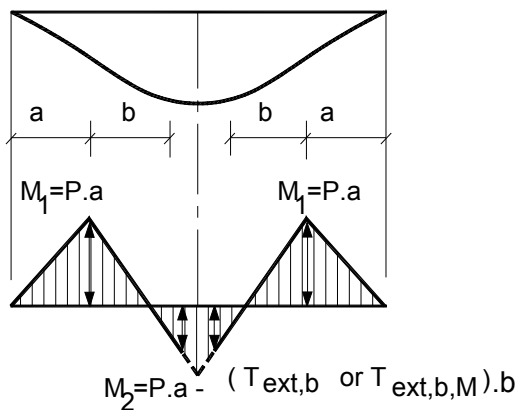
Figure (6.11) Equivalent Tee Stub Connection
