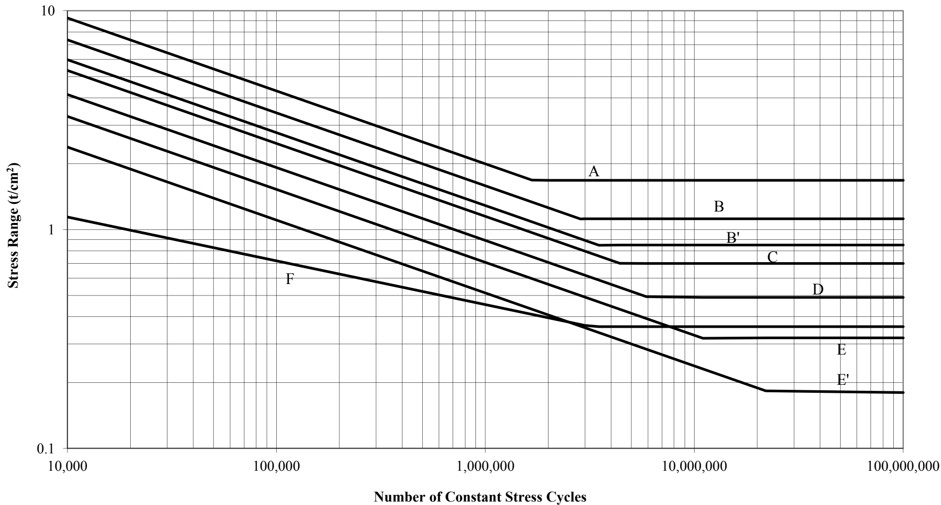
Fig. 3.1. Stress Range Versus Number of Constant Stress Cycles
