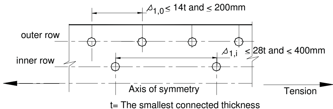
Figure (6.3) Maximum Spacing in Tension Members
