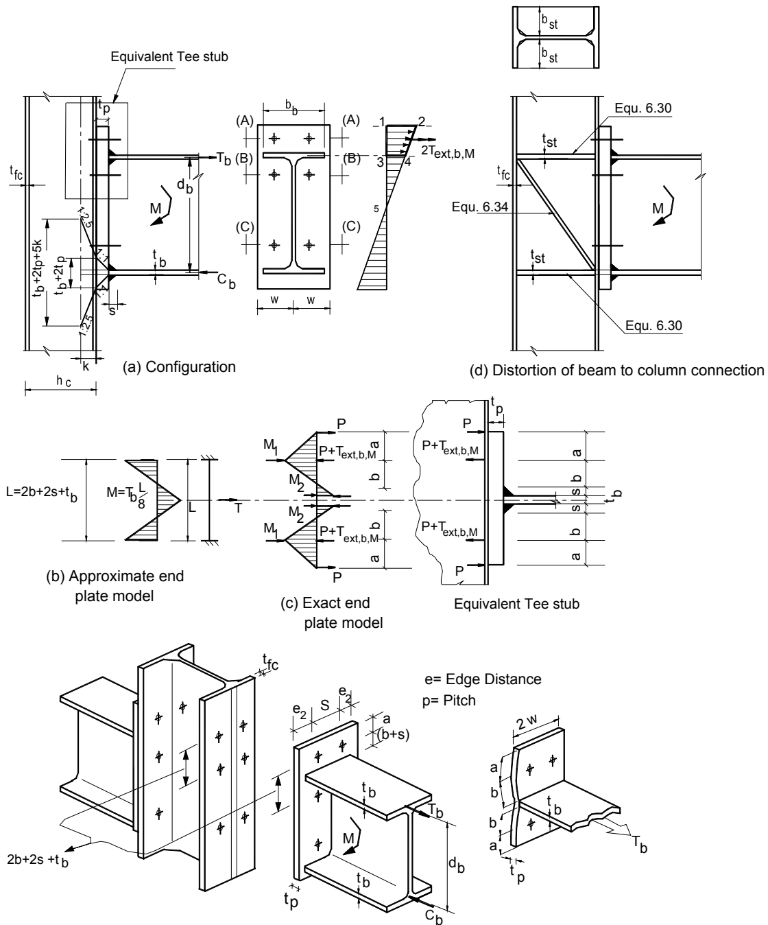
Figure 6.9. Figure (6.12) Determination of The Tee Stub or The End Plate Thickness ( t_p )
