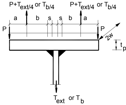
(a) Welded flange
