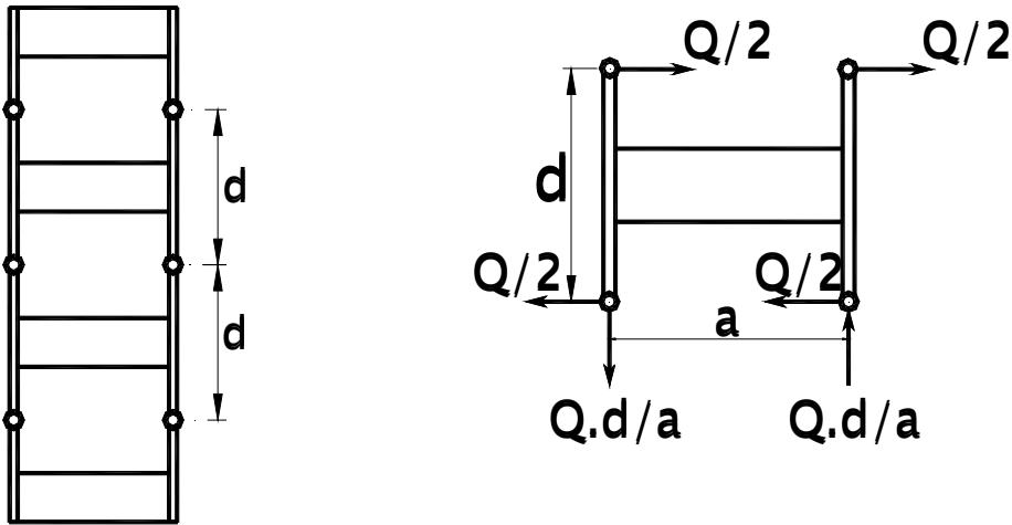
Figure (9.2) Battened Compression Members
