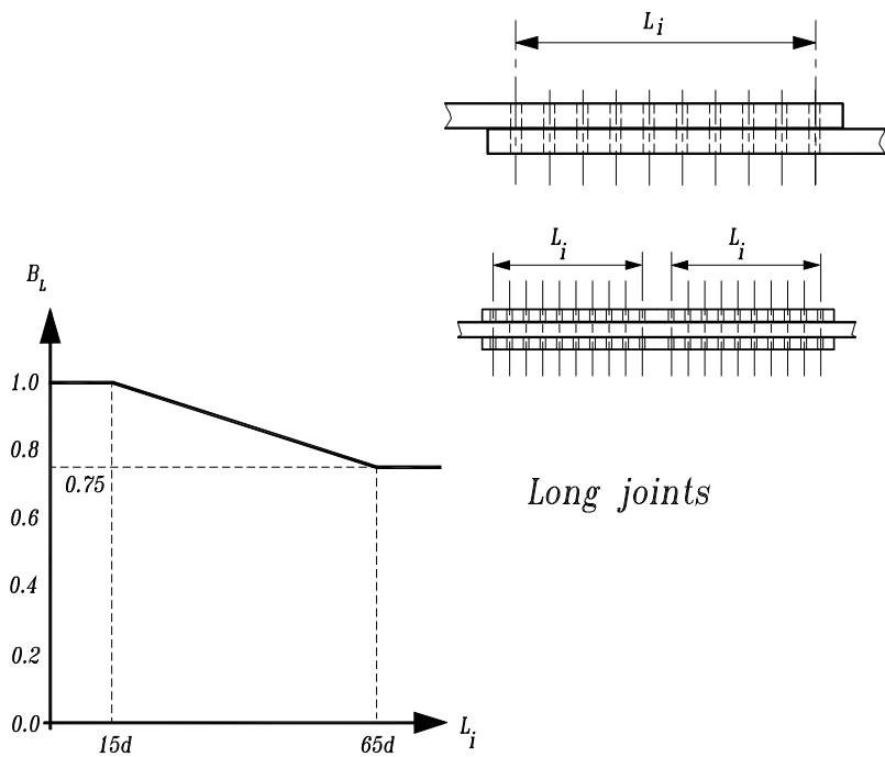
Figure. 6.10. Long joints
