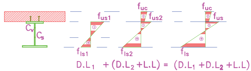
(a) Without Shoring (Case I)
