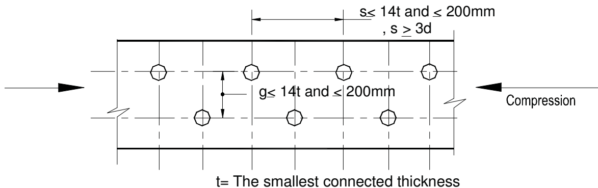
Figure (6.2) Staggered Spacing - Compression
