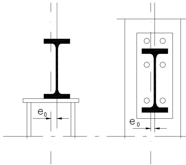
Figure (12.15) Eccentricity of Girder Bearing
