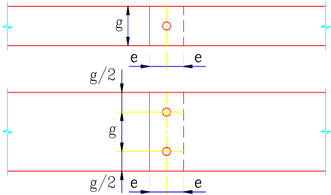
Figure (11.14) Spacing and Edge Distance of Bolts
