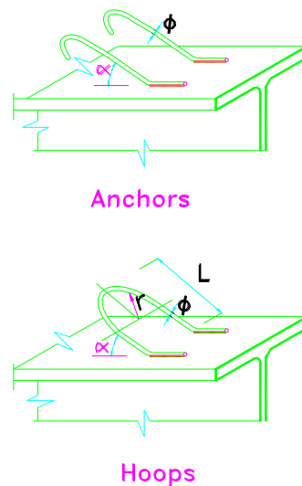
Figure (10.10) Anchor & Hoop Shear Connectors
