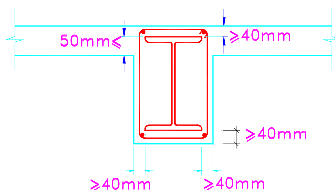
Figure (10.9) Encased Beam
