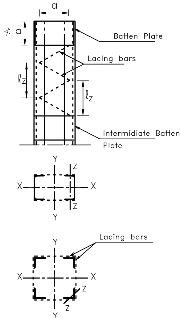
Figure (9.1) Laced Compression Members
