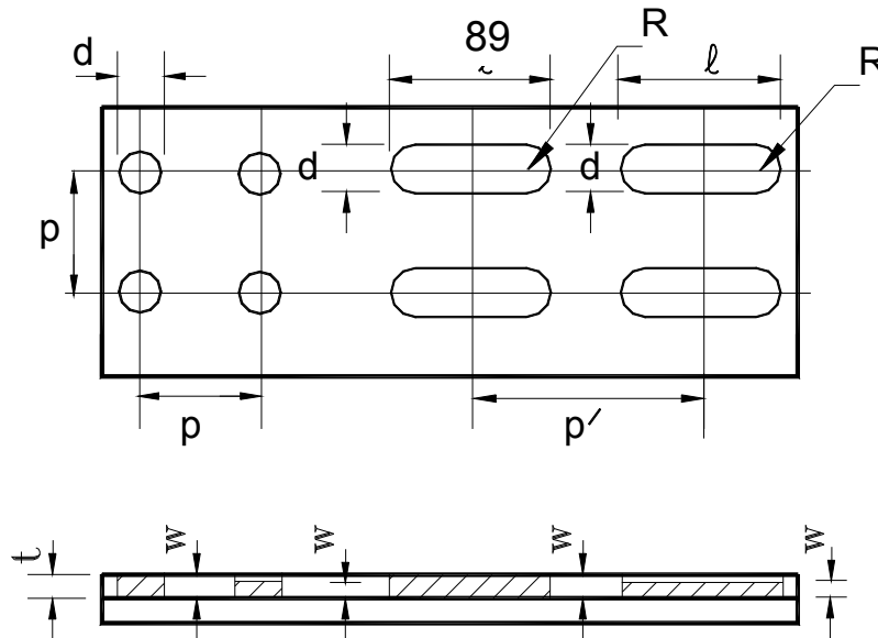
Figure (5.13) Definition of Plug and Slot Welds
