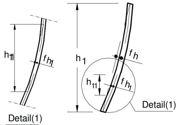
Figure (12.1) Inclination and Deflections of Columns
