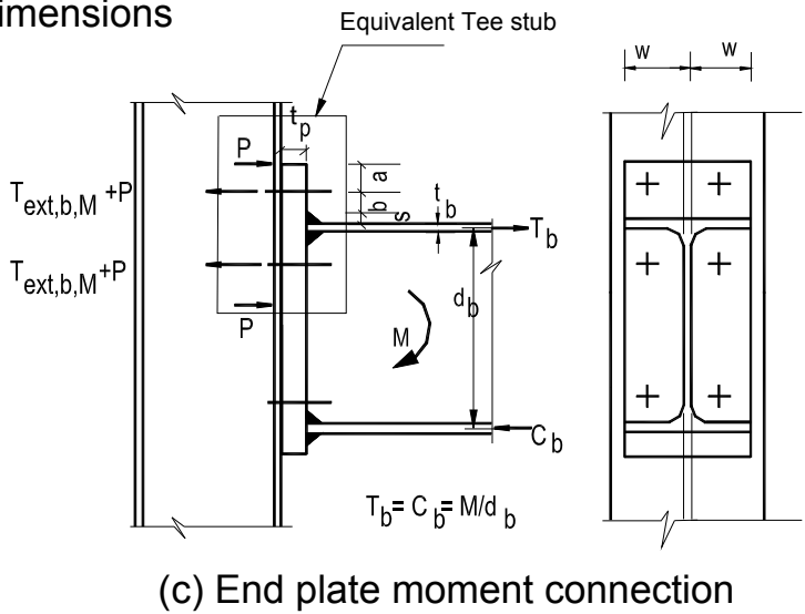
Figure (6.10) Common Types of Connections Producing Prying Forces
