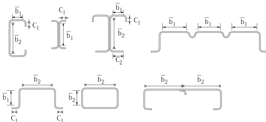
Figure (11.1) Definition of Flat Width of Compression Elements
