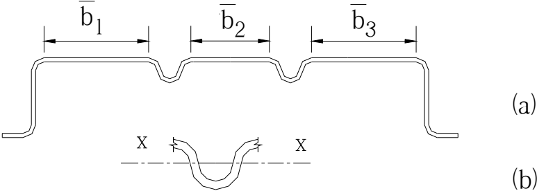
Figure (11.5) Sections with Multiple-Stiffened Compression Elements
