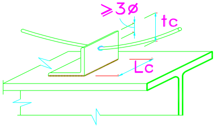
(b) Channel Connectors
