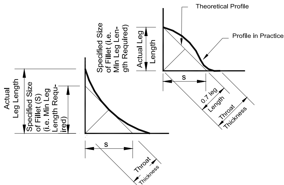
Figure ( 5.9) Definition of Throat in a Fillet Weld
