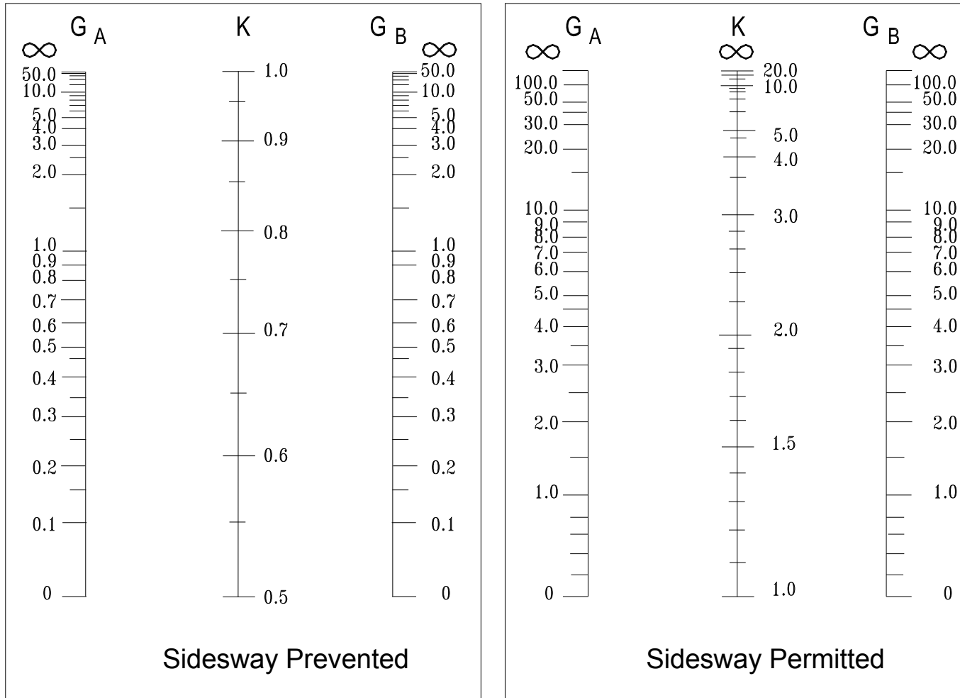
Figure (4.3) Alignment Charts for Buckling Length Factor ( K ) of Columns in Rigid Frames Figure (5.2) Alignment Charts for Effective Length of Columns in Rigid Frames .
