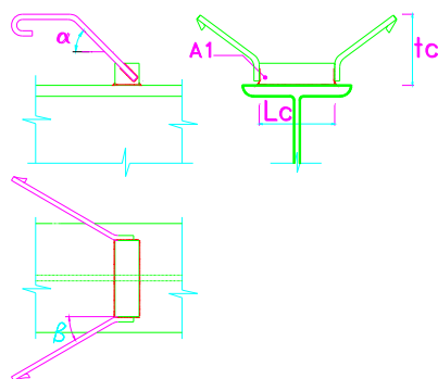
Block Connector with anchor
