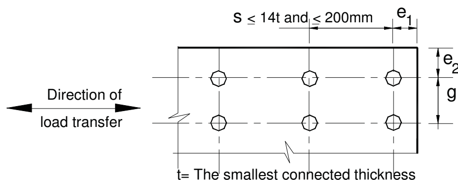
Figure (6.1) Spacing in Tension or Compression Members
