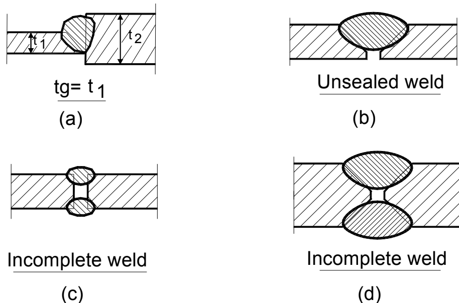
Figure (5.4) Incomplete Penetration and Unsealed Welds
