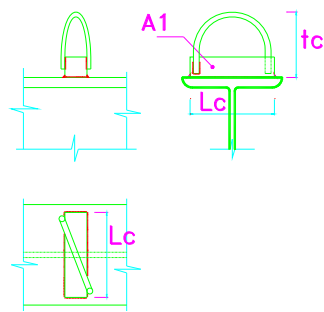
Block Connector with hoop
