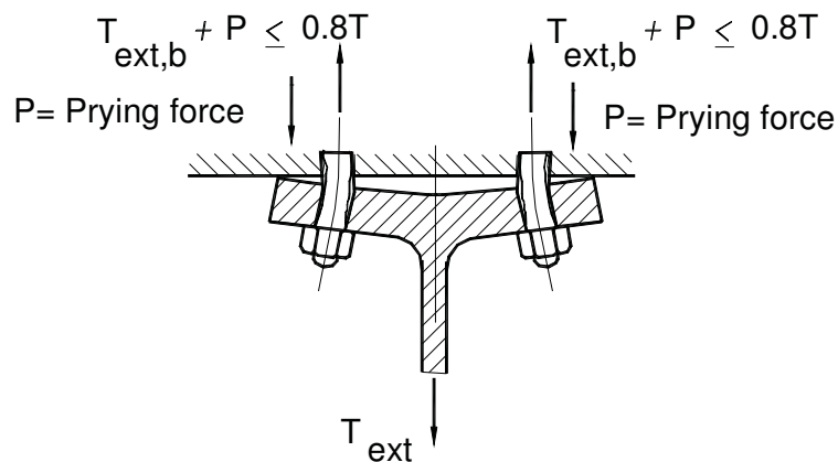
Figure (6.5) Prying Force
