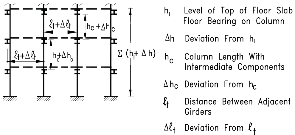
Figure (12.5) Deviation in Height and Length
