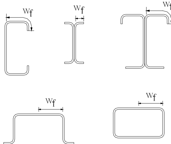
Figure (11.6) Definition of ( w_f ) of Compression Elements
