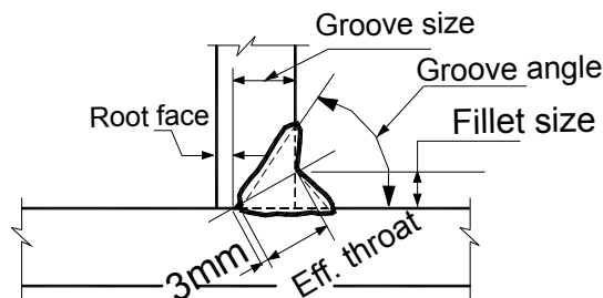
Partial penetration (When reinforcing fillet is specified)
