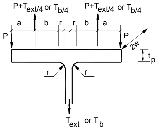
(b) Tee- Stub
