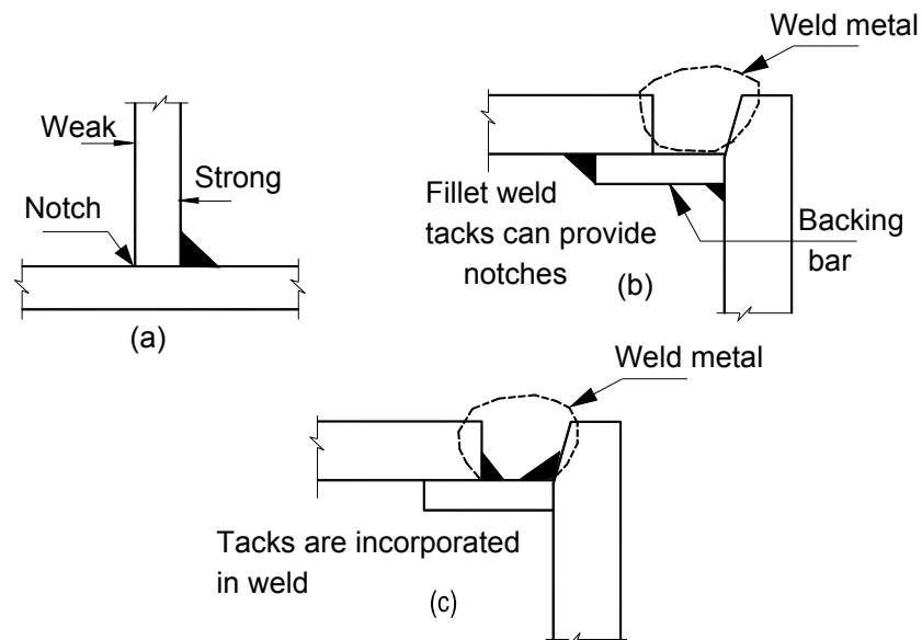
Figure (5.15) Notches and Brittle Fracture
