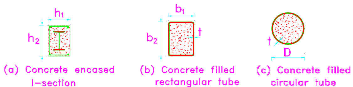
Figure (10.15) Sections for Composite Columns
