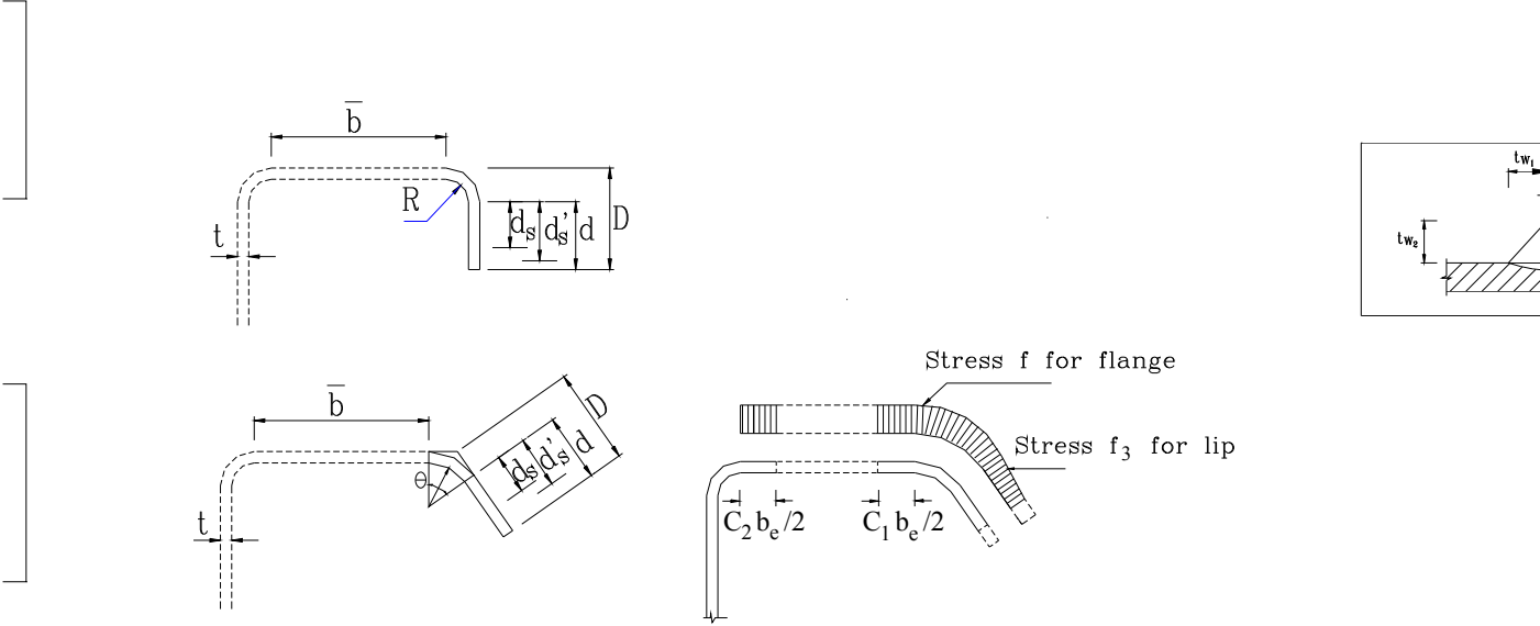
Figure (11.3) Elements with Edge Stiffener
