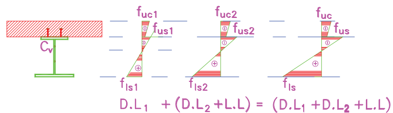
(a) With Shoring (Case II)
