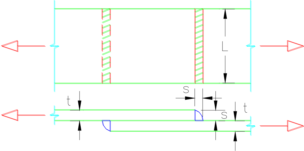
Figure (11.10) Fillet Welds
