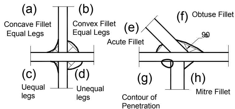
Figure ( 5.7) Fillet Weld Configurations
