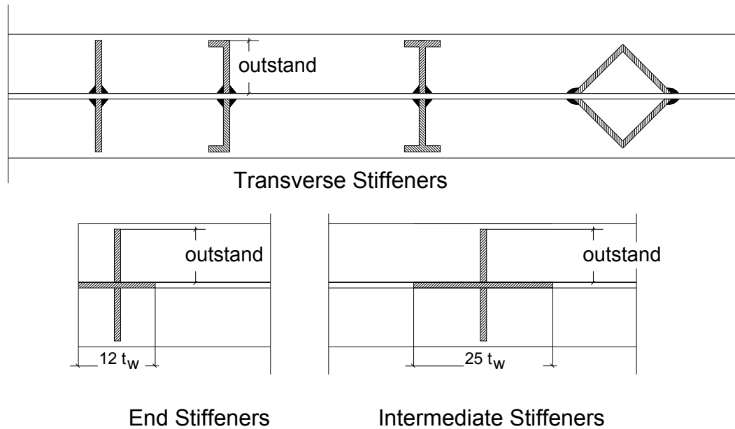
Figure (7.1) Intermediate Transverse Stiffeners
