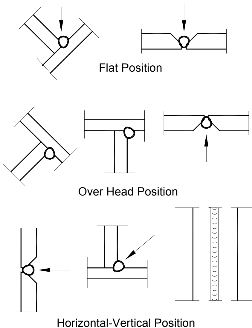
Figure (5.1) Welding Positions
