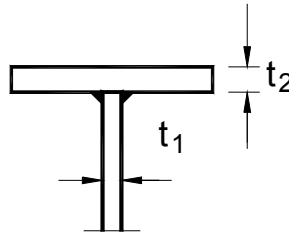
Figure( 5.10) Thickness of Plates to be Welded
