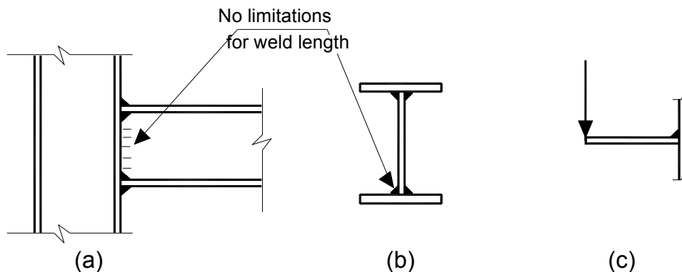
Figure (5.11) Different Locations of Fillet Welds
