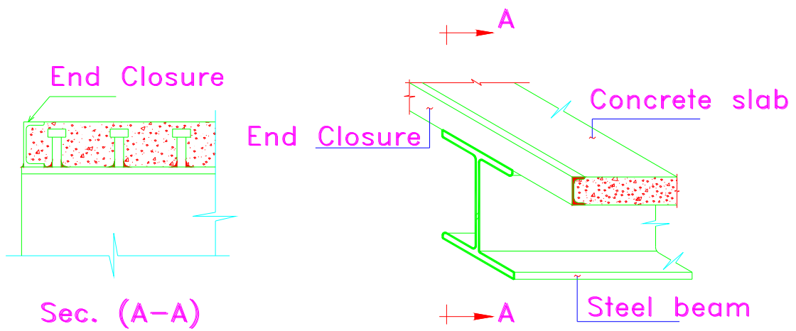
Figure (10.8) End Closure for Concrete Slab
