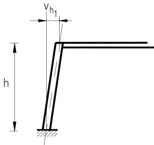
Figure (12.12) Inclination of Column in a Single-Storey Building
